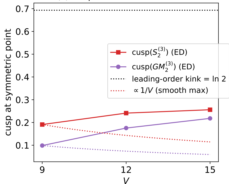
(c) Cusp does not shrink with V
