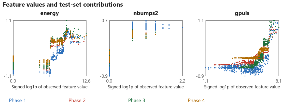
Figure 3. Values and TreeSHAP contributions for the three globally leading features. Colours identify test phases; horizontal values use signed log1p for display, and vertical values are raw log-odds contributions.
