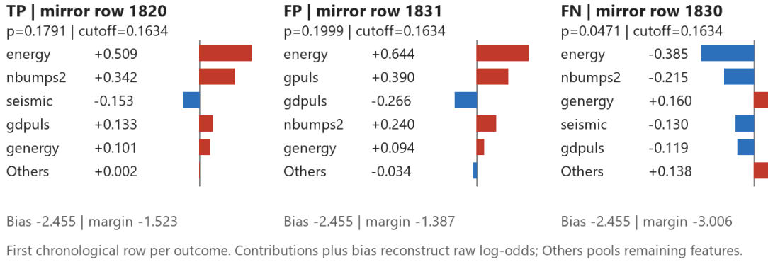
Figure 4. Earliest holdout true-positive, false-positive and false-negative cases under the 10 percent reference budget. IDs are one-based mirror rows; raw log-odds contributions, including Other features, sum with the bias to the margin.
