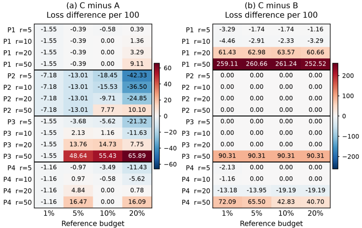
Figure 1. Fixed XGBoost loss contrasts for every phase, cost and capacity budget. Negative values favor C on the stated relative loss. Panels use separate color scales; cell values are rounded to two decimals. P1 to P4 identify test phases, r is the assumed missed-shift cost, and panel letters identify the compared rules.
