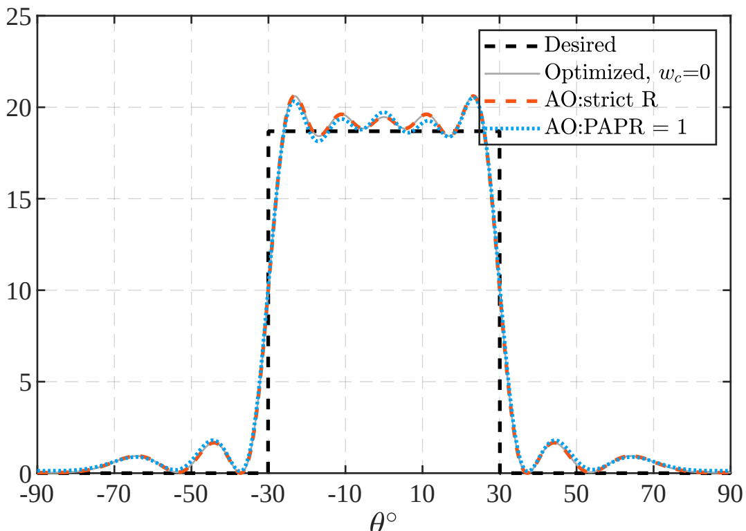
Beampattern
