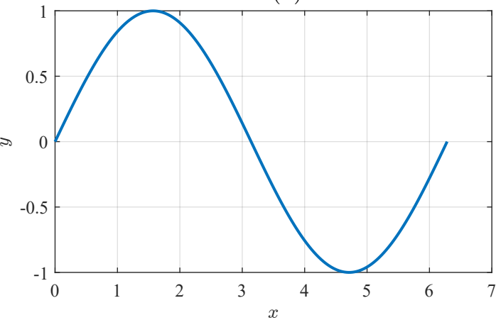
\sin(x)
