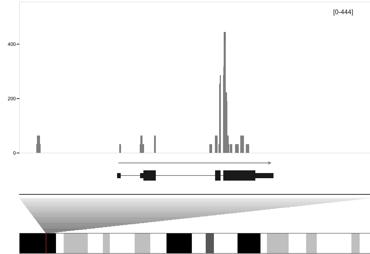
Zscan4c | chr7:11,002,745-11,013,547
