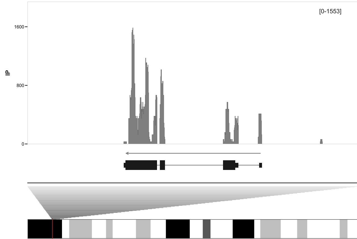
Zscan4b | chr7:10,897,740-10,908,050
