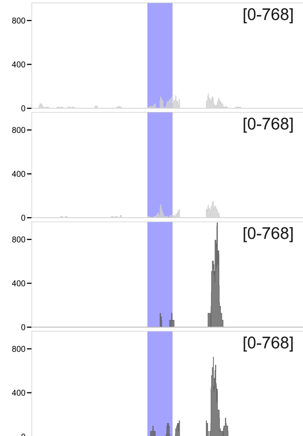
Myc | chr15:61,982,391-61,993,374
