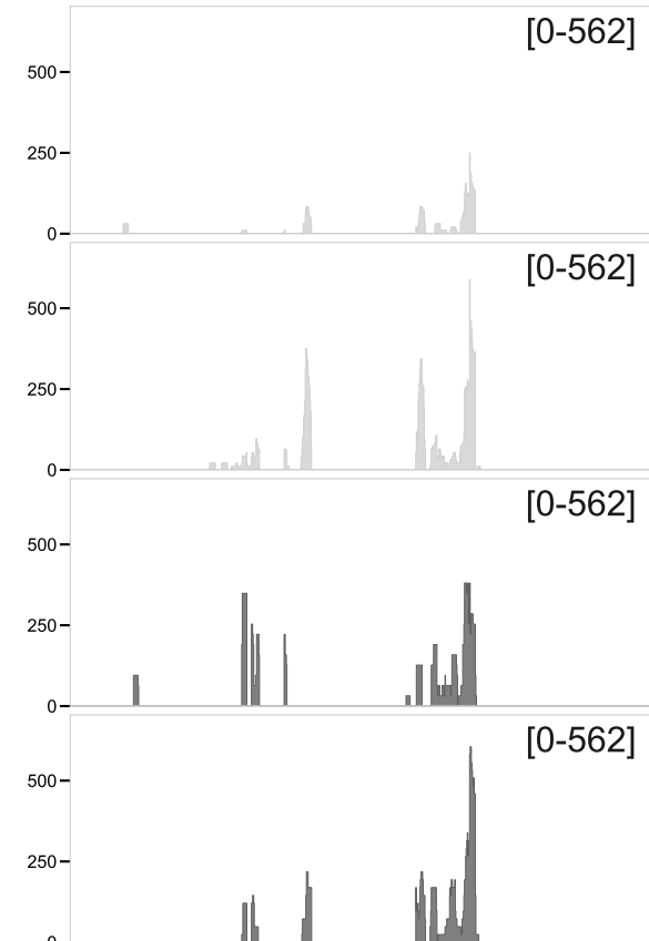
Zscan4f | chr7:11,394,915-11,405,318
