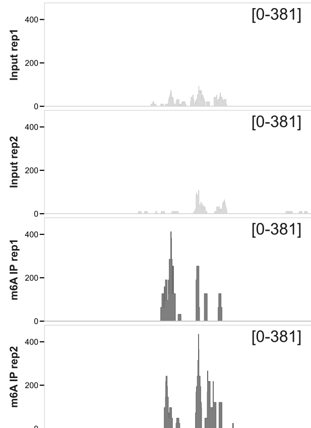
Jun | chr4:95,046,034-95,055,222
