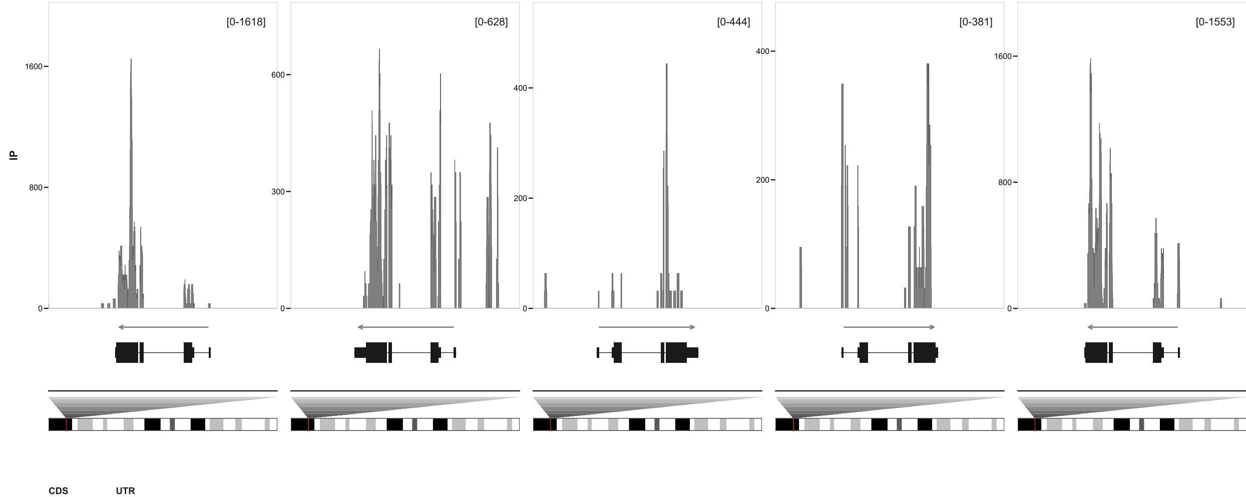
Zscan4e | chr7:11,303,378-11,313,682
