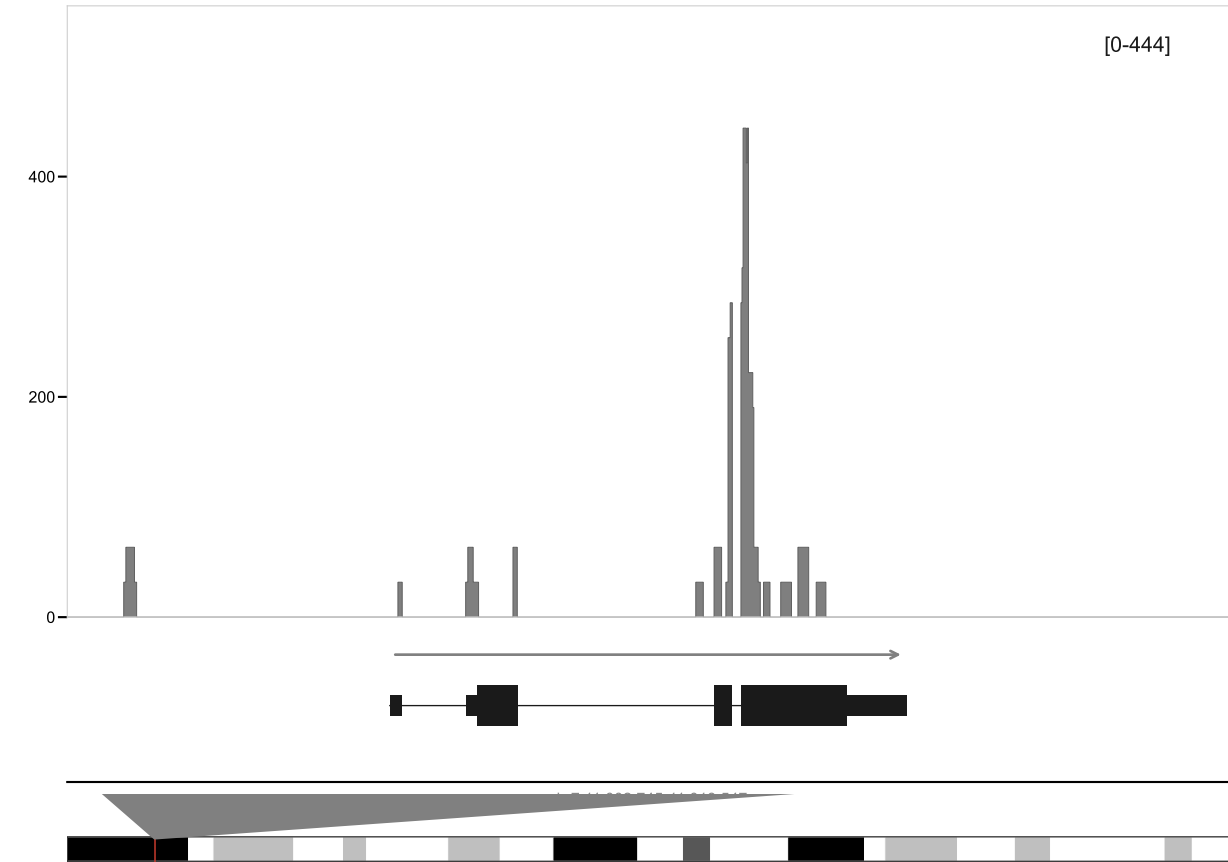
Zscan4c | chr7:11,002,745-11,013,547
