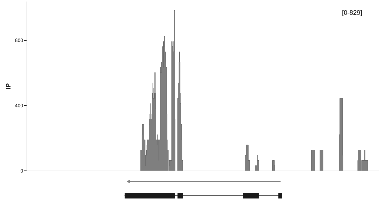
Zscan4a | chr7:10,791,242-10,802,057
