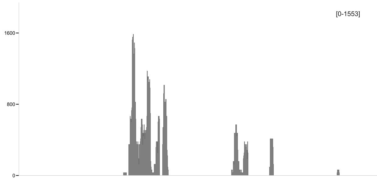
Zscan4b | chr7:10,897,740-10,908,050
