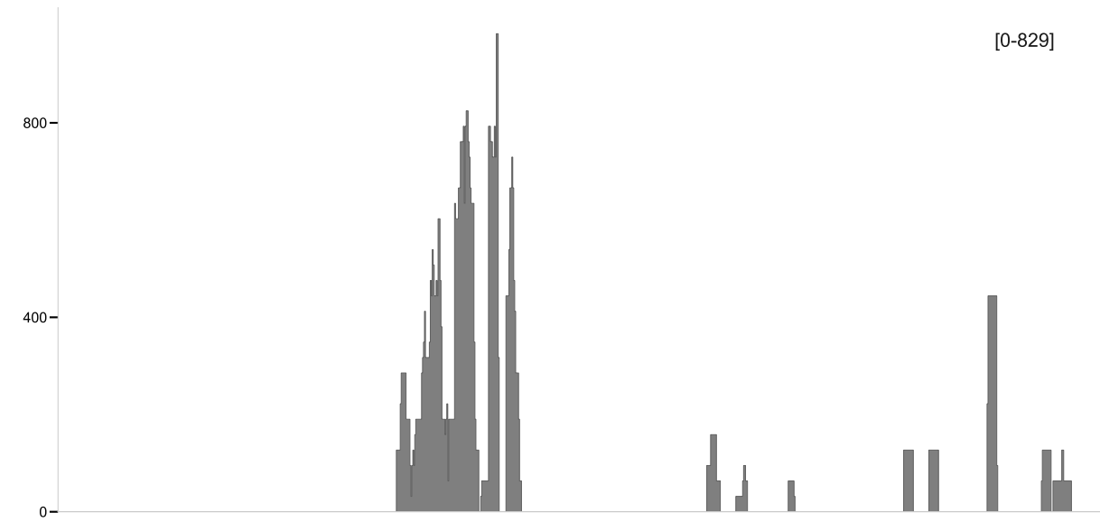
Zscan4a | chr7:10,791,242-10,802,057
