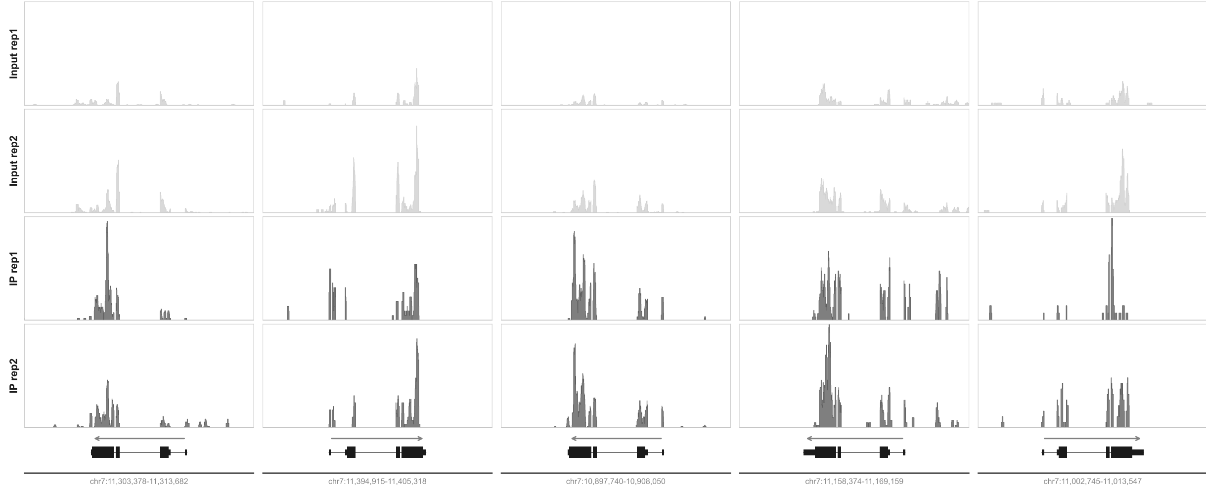
Zscan4e | chr7:11,303,378-11,313,682
