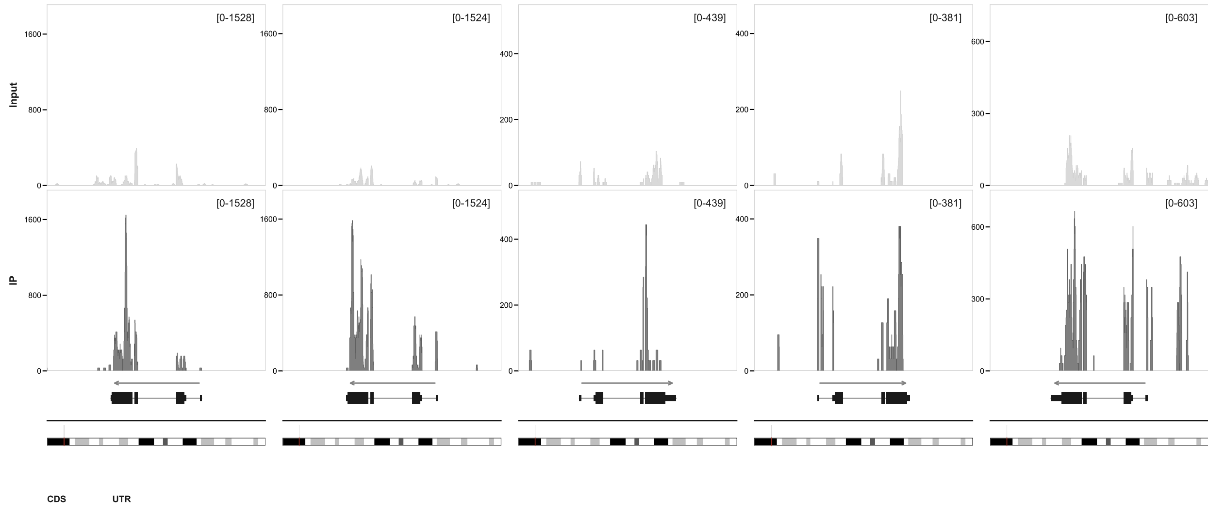
Zscan4e | chr7:11,303,378-11,313,682
