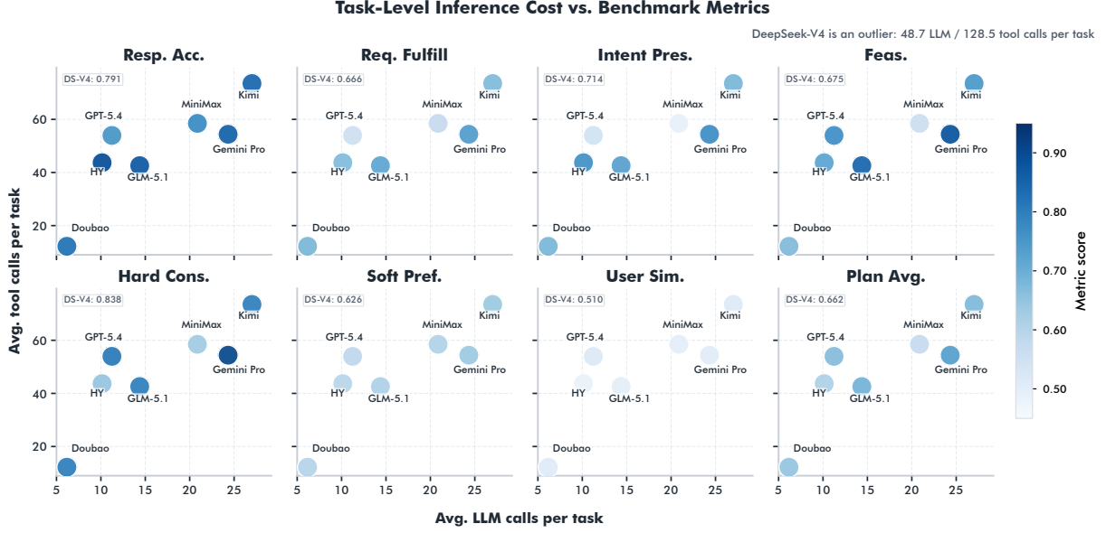
Figure 9: Task-level inference cost and planning performance across benchmark metrics
