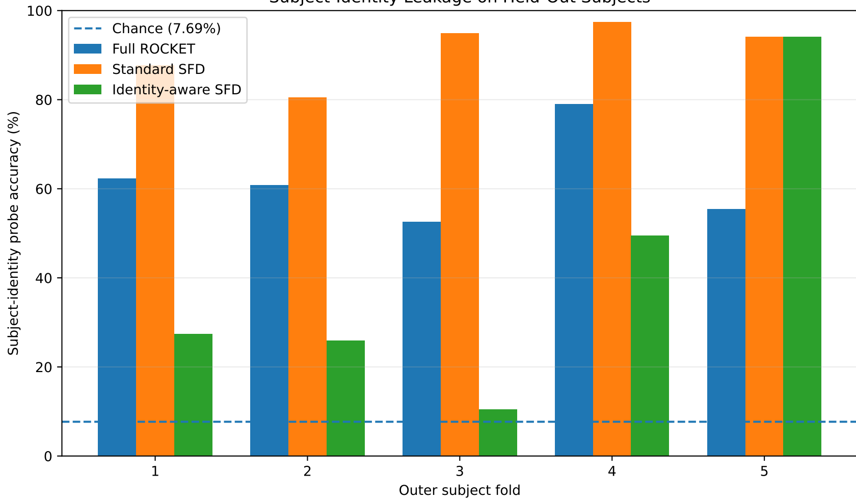
Subject-Identity Leakage on Held-Out Subjects
