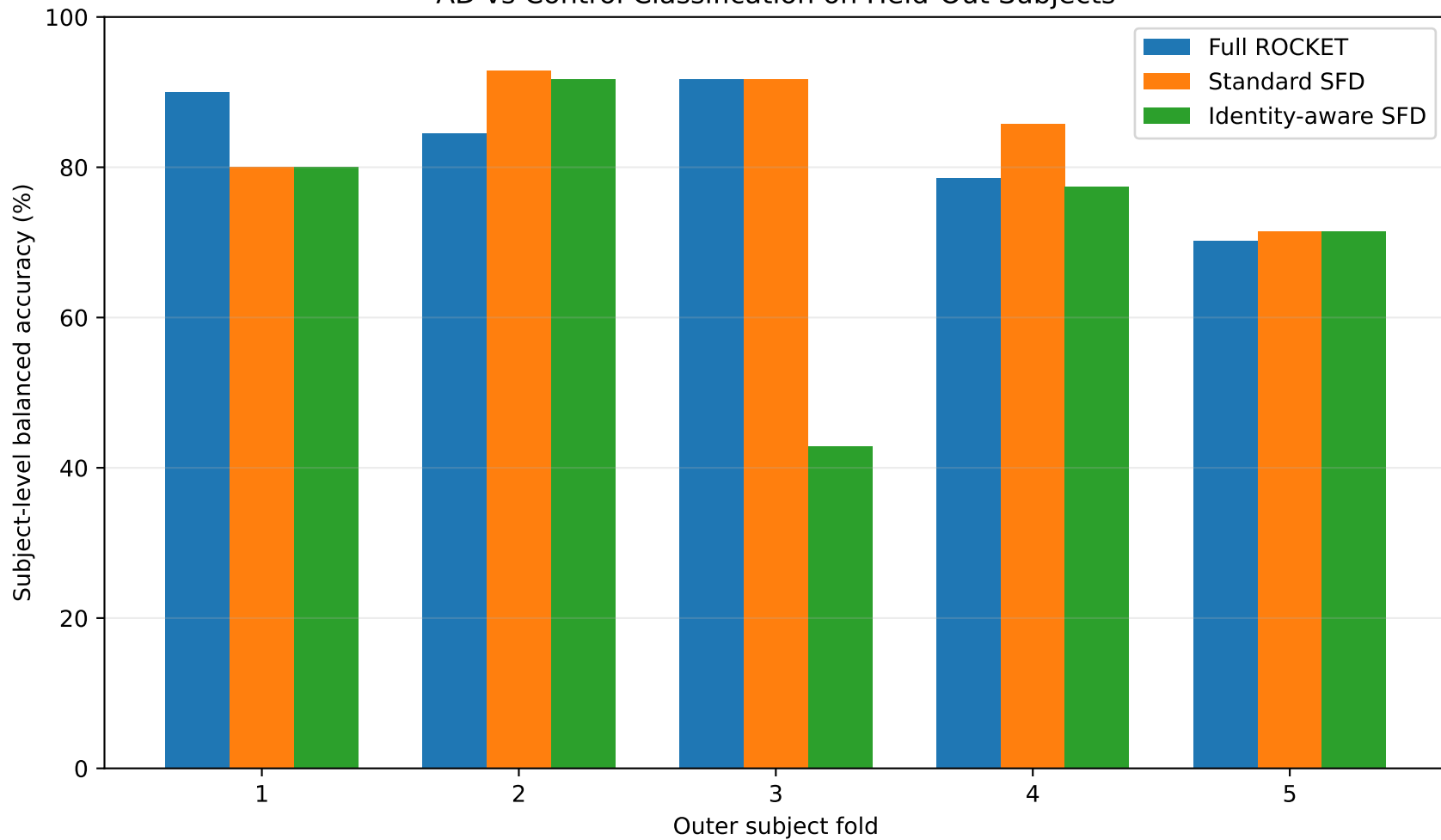
AD vs Control Classification on Held-Out Subjects
