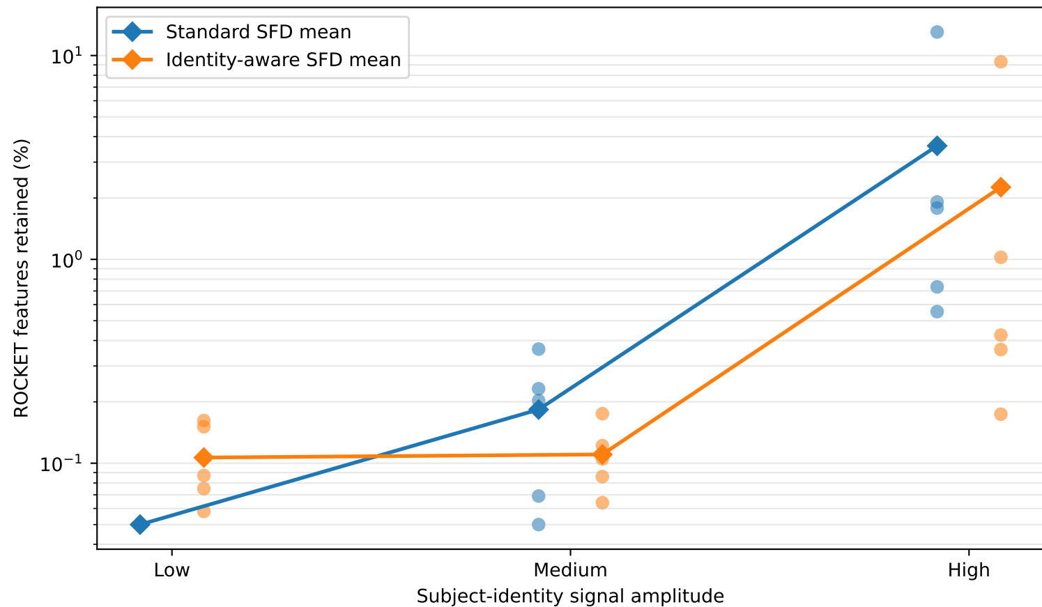
Feature retention
