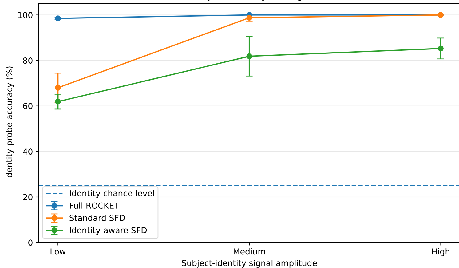
Subject-identity leakage
