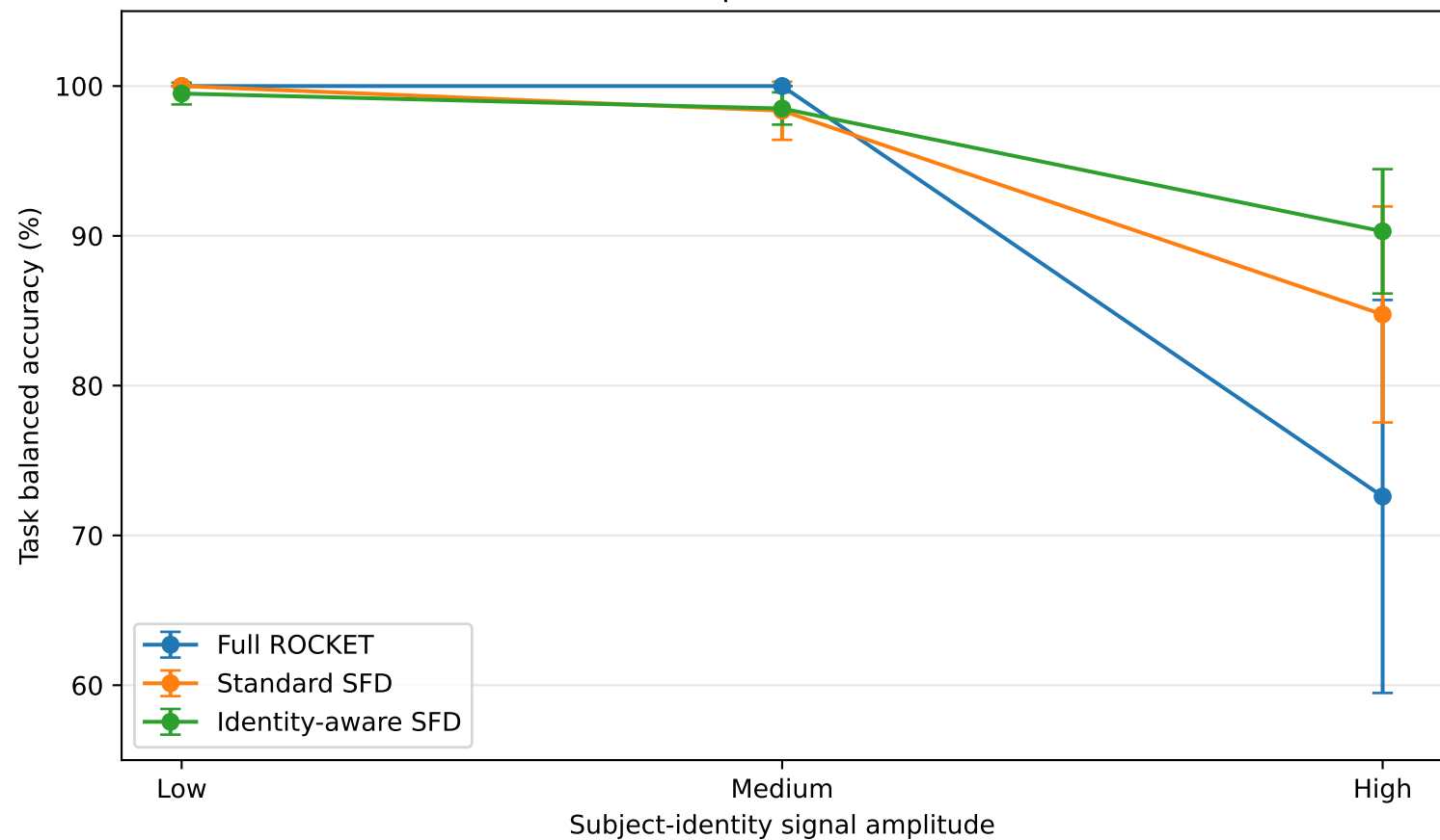
Task performance
