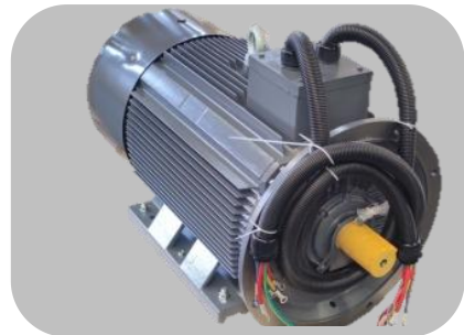
Special TB and lead wire
