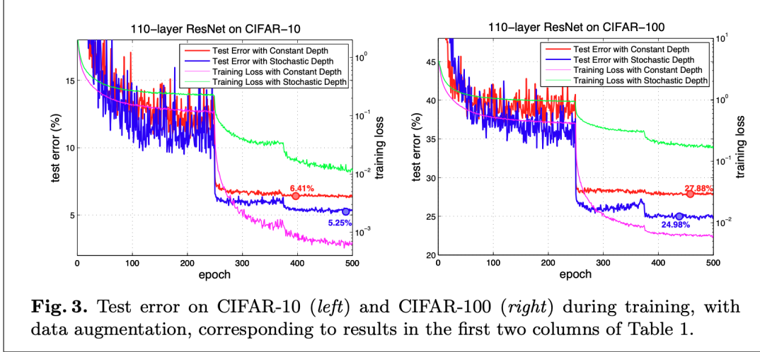
Figure 1: Figure 3 (left) from Huang et al. [1]: test error and training loss for the 110-layer ResNet on CIFAR-10. Constant depth achieves 6.41%; stochastic depth achieves 5.25%.
