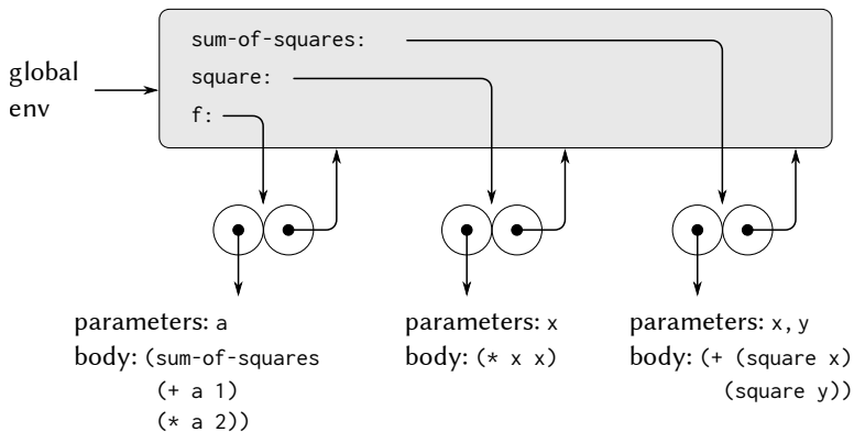
Figure 3.4: Procedure objects in the global frame.
