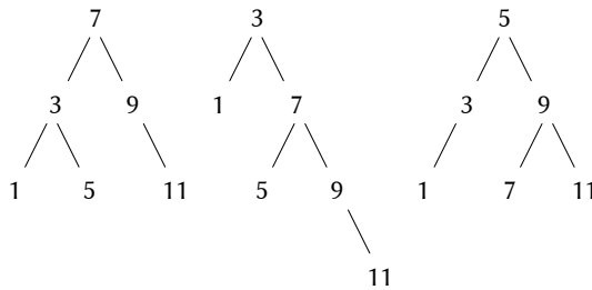
Figure 2.16: Various binary trees that represent the set \{1, 3, 5, 7, 9, 11\} .
