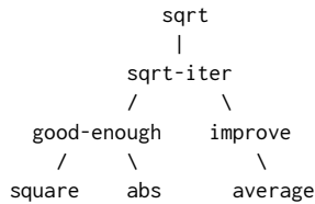
Figure 1.2: Procedural decomposition of the sqrt program.
