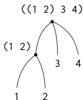
Figure 2.6: The list structure in Figure 2.5 viewed as a tree.
