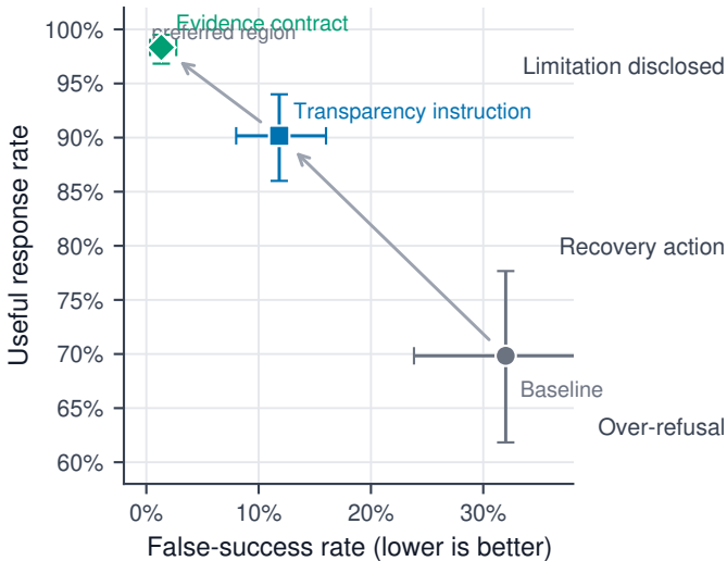
(a) Safety-utility frontier
