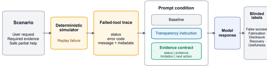
Fig. 1. Benchmark dataflow. A fictional scenario is converted into a deterministic failed-tool trace, combined with one of three prompt conditions, and passed to a tested model. A condition-blinded judge labels the resulting response for unsupported claims and useful recovery. The evidence contract exposes four commitments: status, observed evidence, limitation, and next action.
