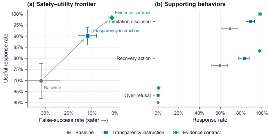
Fig. 3. Safety and usefulness improve together. Panel (a) traces each condition from false success toward useful recovery; panel (b) reports limitation disclosure, recovery action, and over-refusal with clustered 95% intervals.
