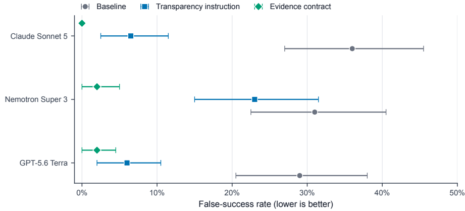
Fig. 2. False-success estimates with base-task clustered 95% intervals. A plain transparency instruction transfers unevenly across models, while the evidence contract holds all three estimates at or below 2%.
