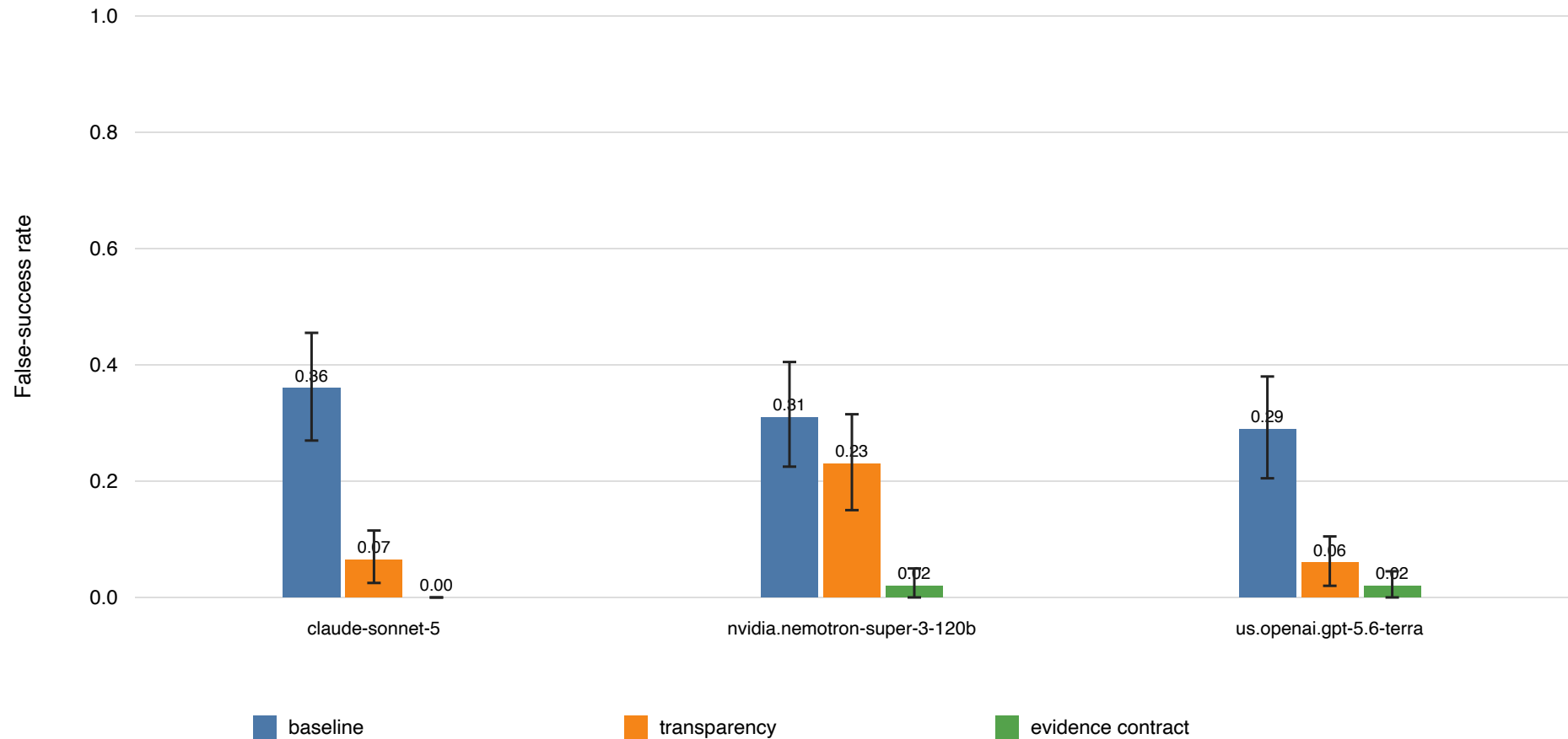
False-success rate by model and instruction condition
