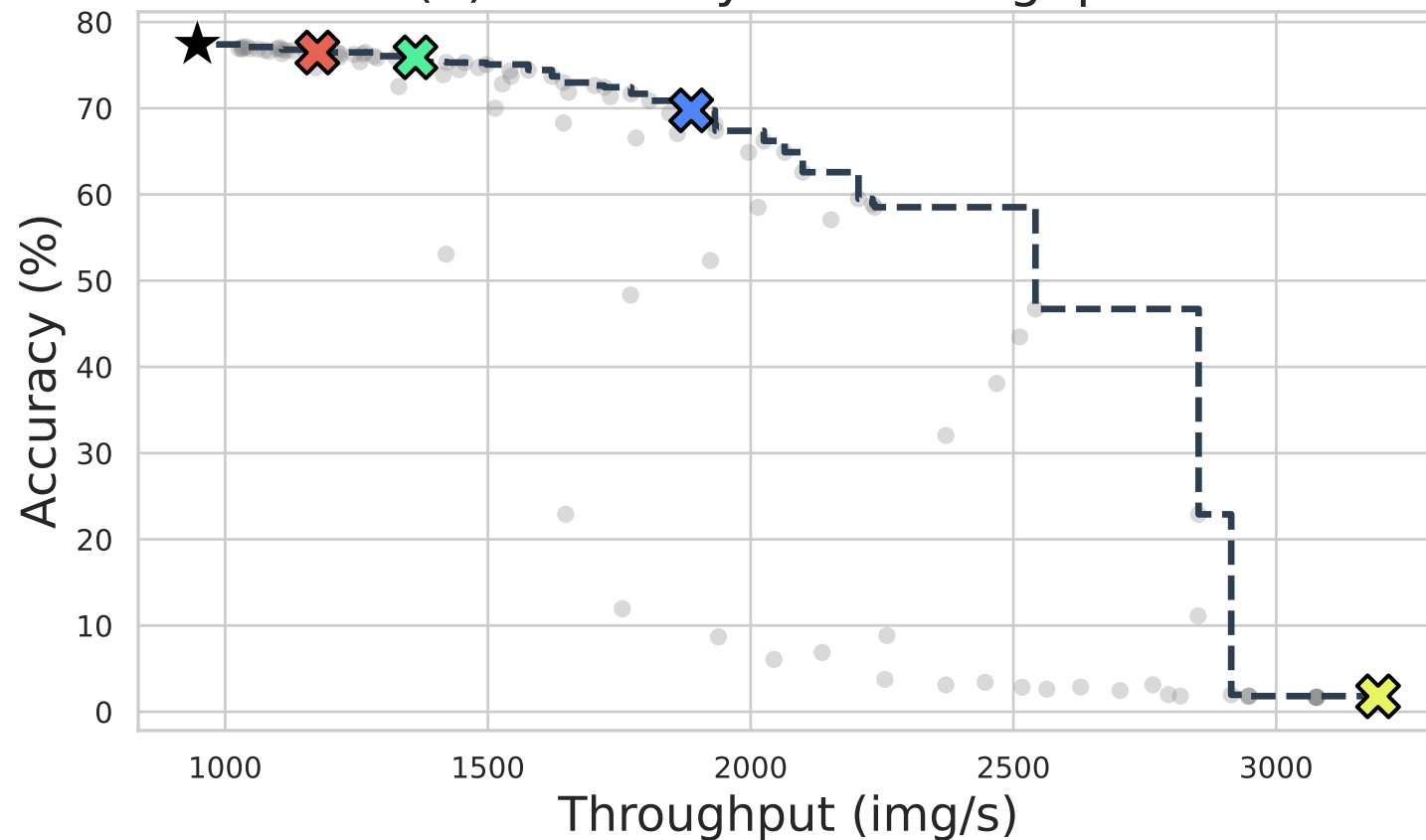
(a) Accuracy vs. Throughput
