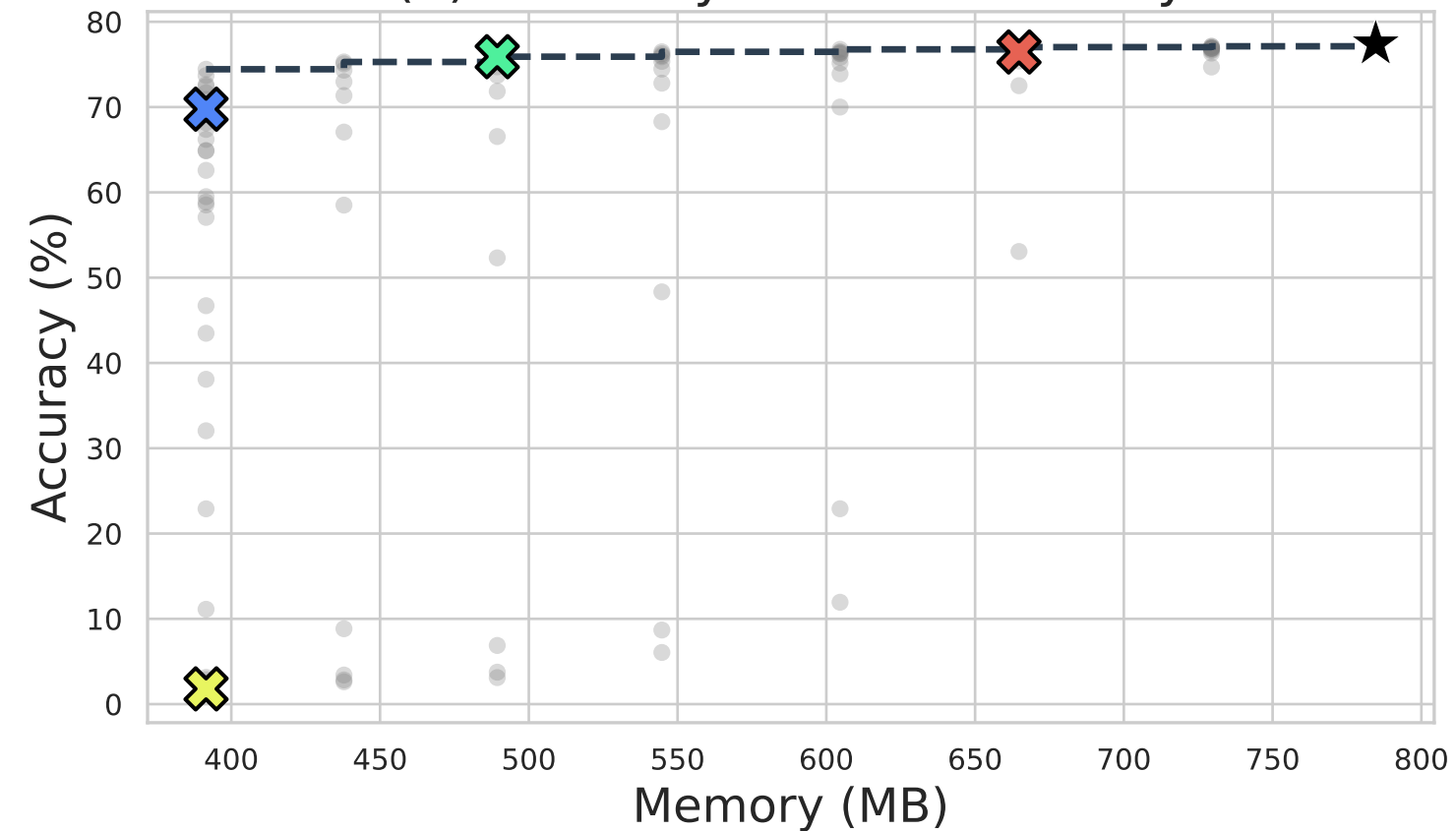
(b) Accuracy vs. Peak Memory
