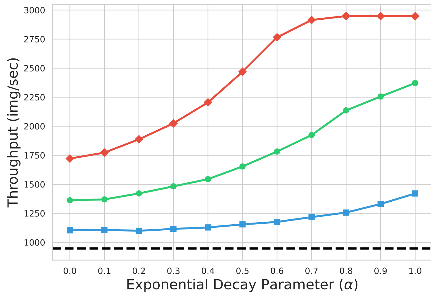
(b) Throughput [GPU | BS=128]
