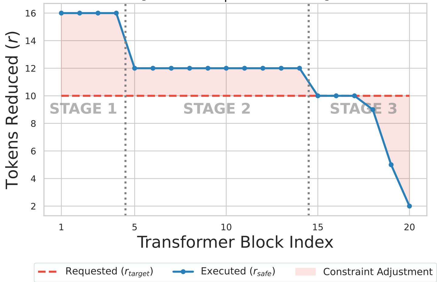
(a) Constant ( r_{const} = 10 ) [Total: 230 | Acc: 71.01%]
