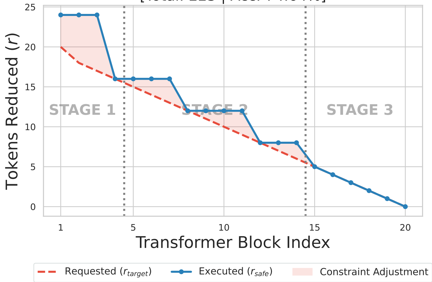
(b) Linear ( r_{lin} = 10 ) [Total: 223 | Acc: 74.64%]
