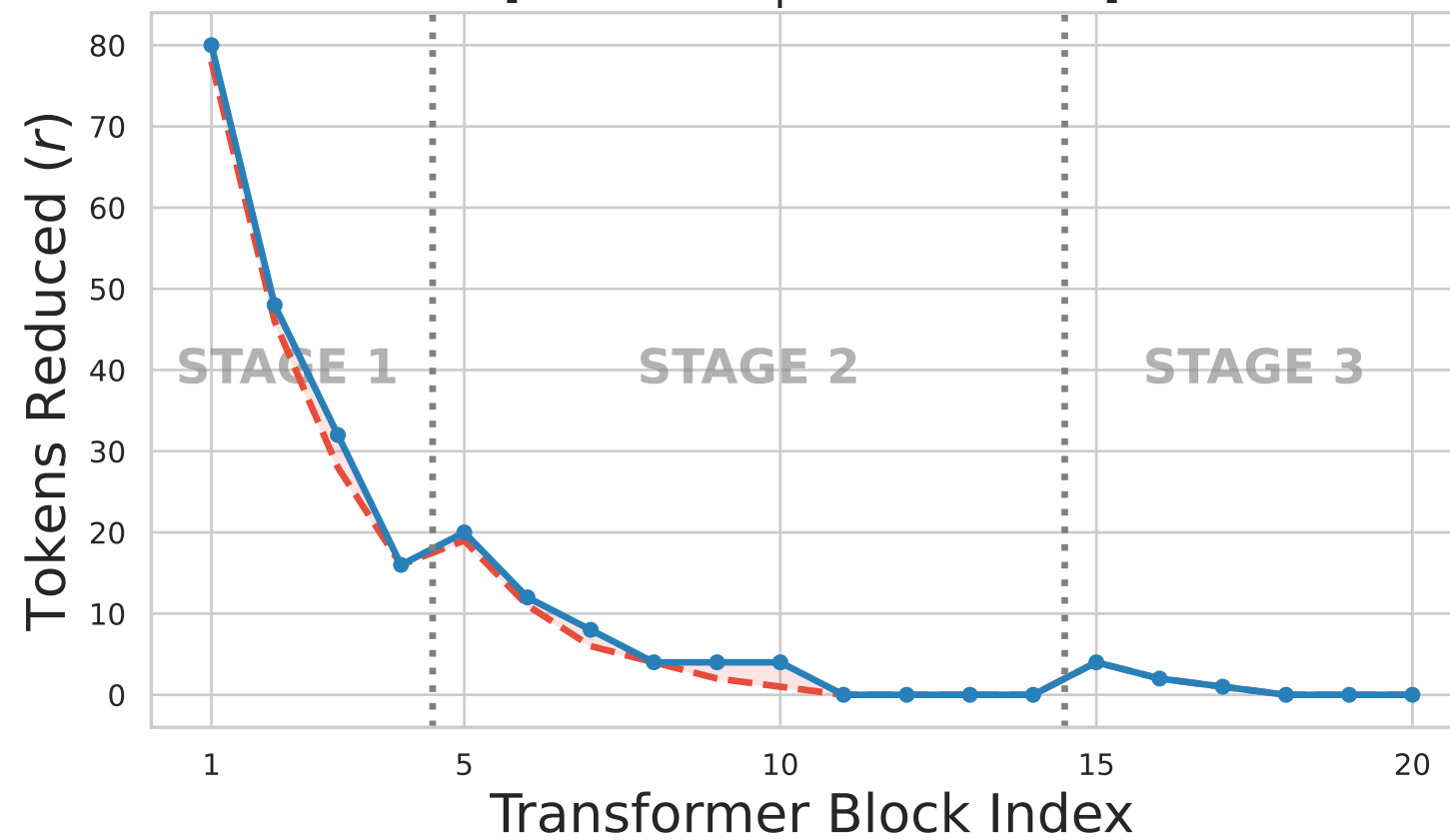
(c) Exponential ( r_{init} = 0.10, \alpha = 0.6 ) [Total: 235 | Acc: 76.35%]
