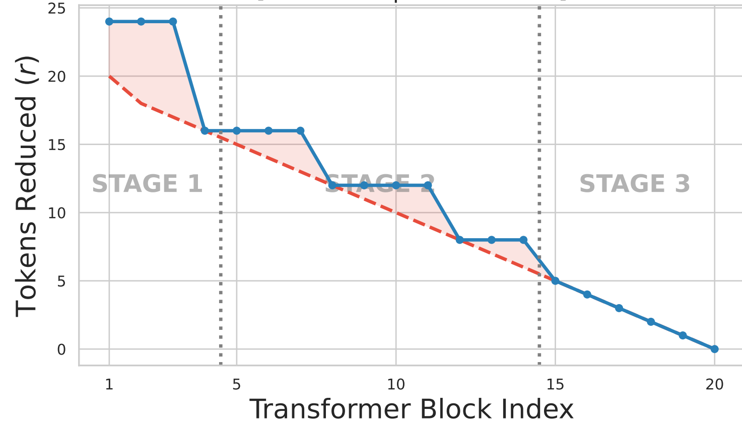
(b) Linear ( r_{lin} = 10 ) [Total: 223 | Acc: 74.64%]
