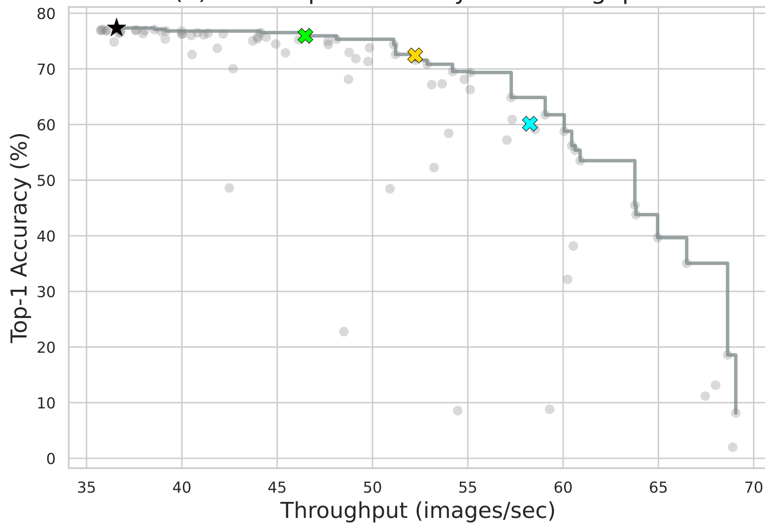
(a) CPU: Top-1 Accuracy vs. Throughput
