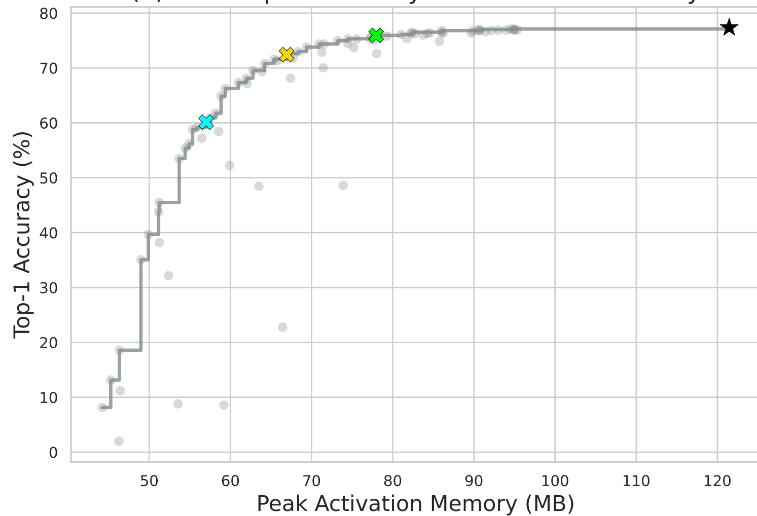
(b) CPU: Top-1 Accuracy vs. Activation Memory
