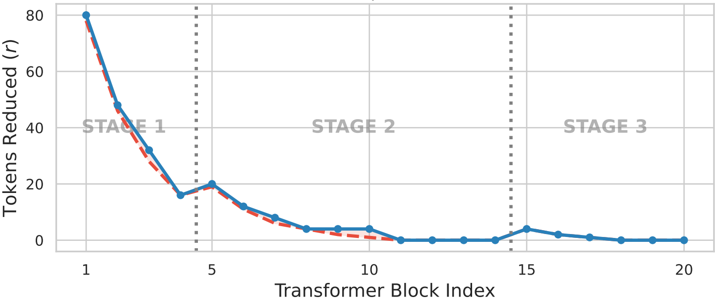
(c) Exponential ( r_{init} = 0.10, \alpha = 0.6 ) [Total: 235 | Acc: 76.35%]
