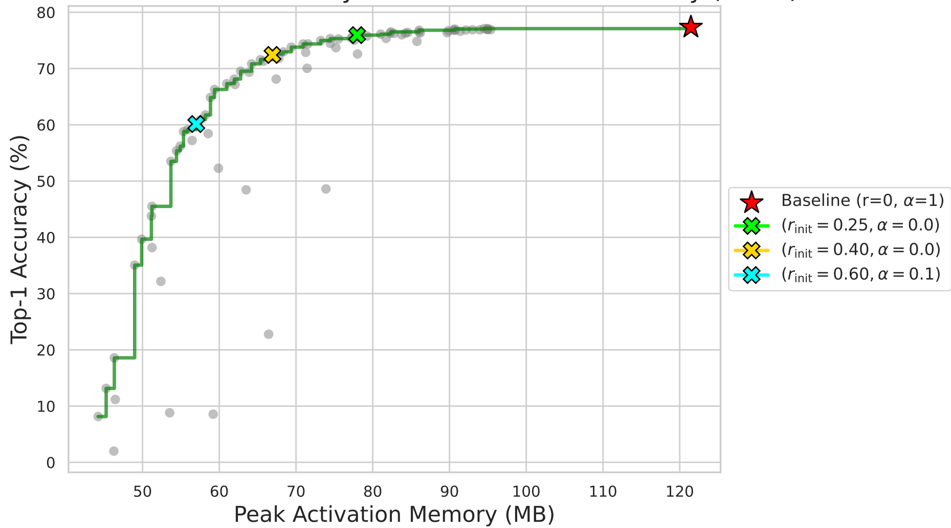
CPU Pareto Frontier: Accuracy vs. Peak Activation Memory (BS=1)
