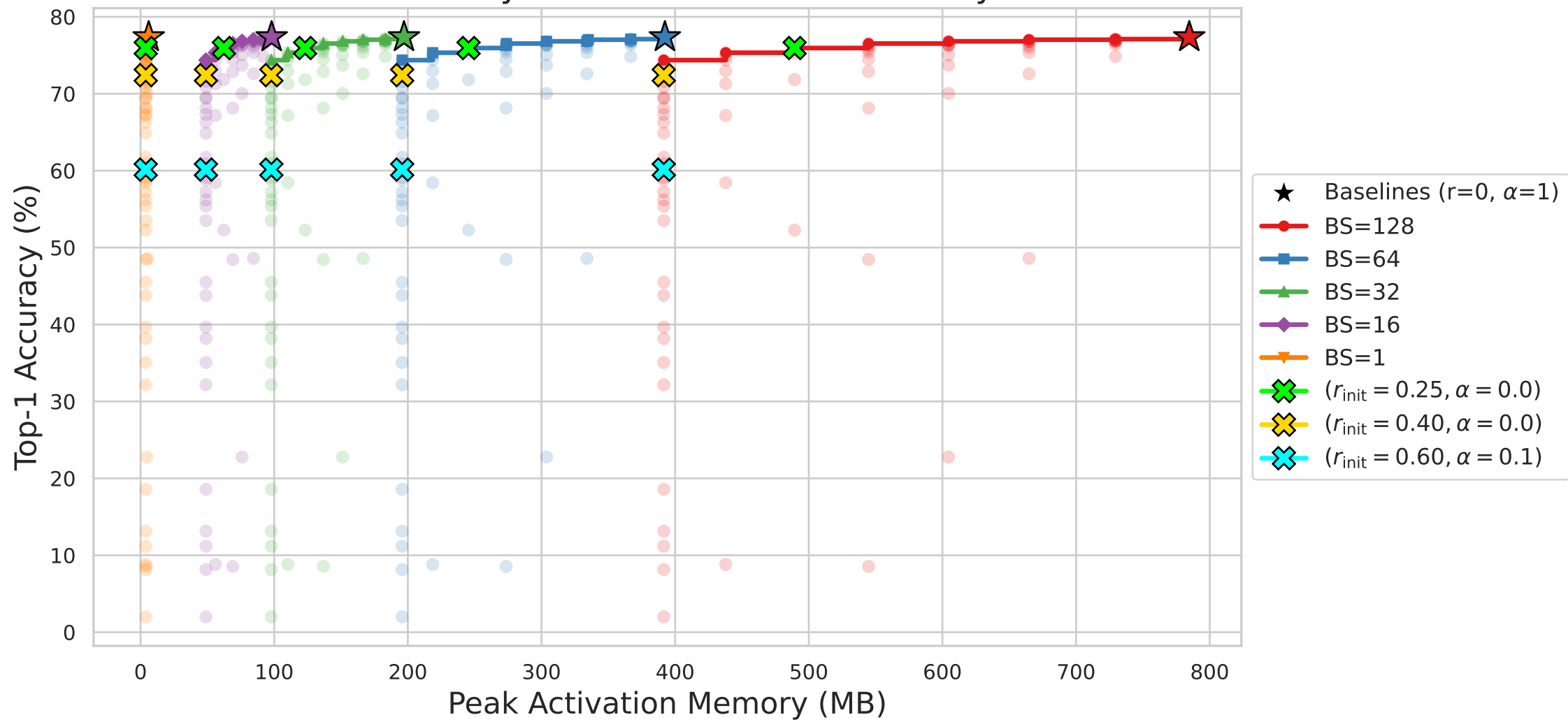
GPU Pareto Frontier: Accuracy vs. Peak Activation Memory across Batch Sizes
