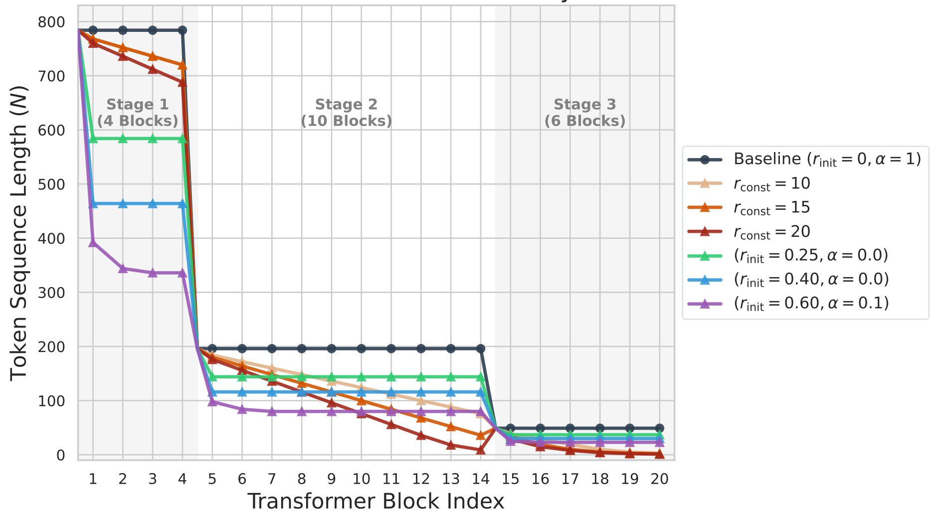
SReT Token Reduction: Constant vs. Dynamic
