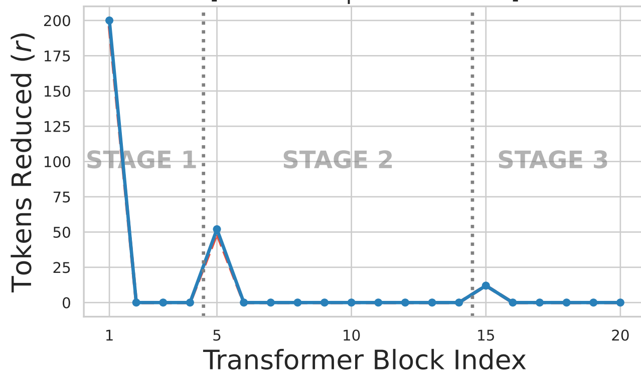
(d) Exponential ( r_{init} = 0.25, \alpha = 0.0 ) [Total: 264 | Acc: 75.95%]
