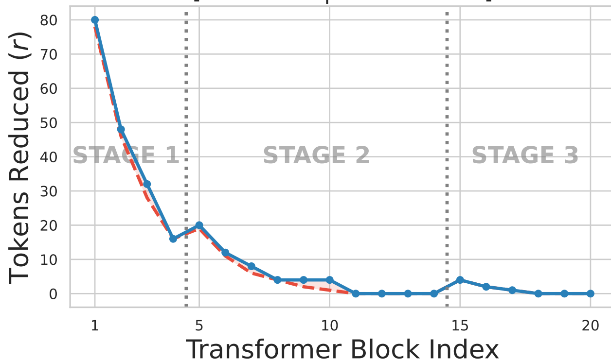
(c) Exponential ( r_{init} = 0.10, \alpha = 0.6 ) [Total: 235 | Acc: 76.35%]
