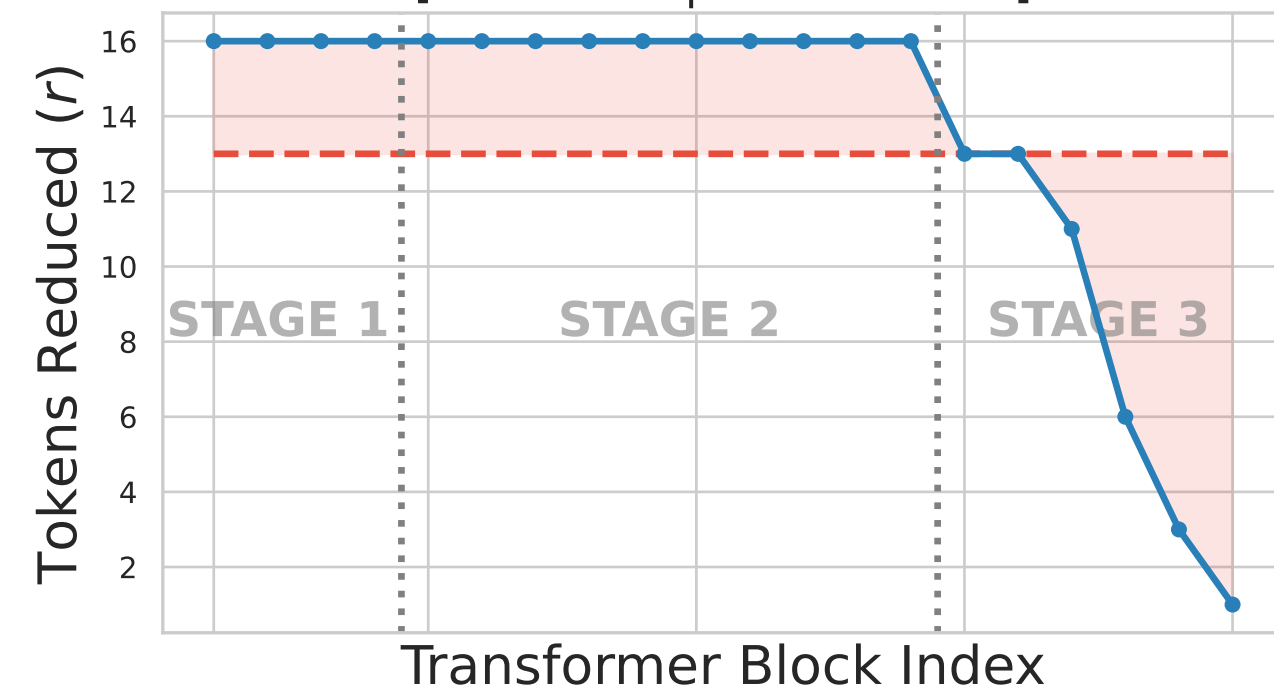
(a) Constant ( r_{const} = 13 ) [Total: 271 | Acc: 61.12%]
