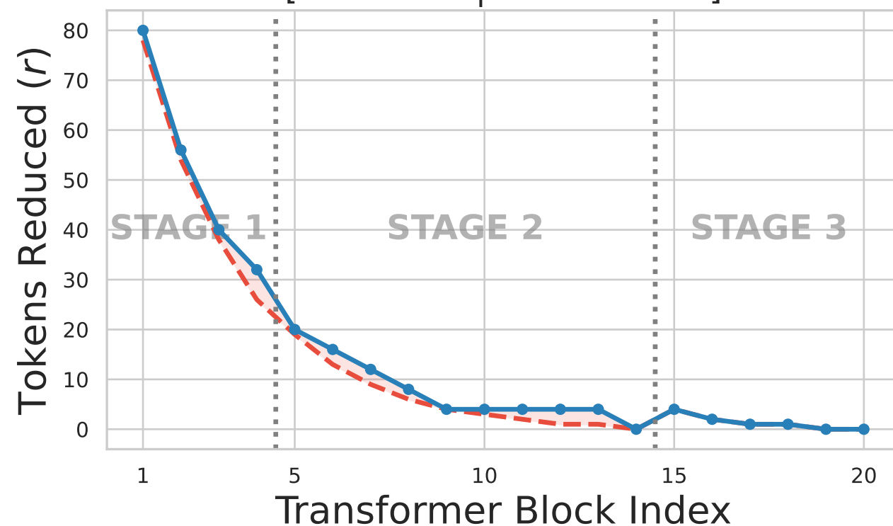
(d) Exponential ( r_{init} = 0.10, \alpha = 0.7 ) [Total: 292 | Acc: 75.95%]
