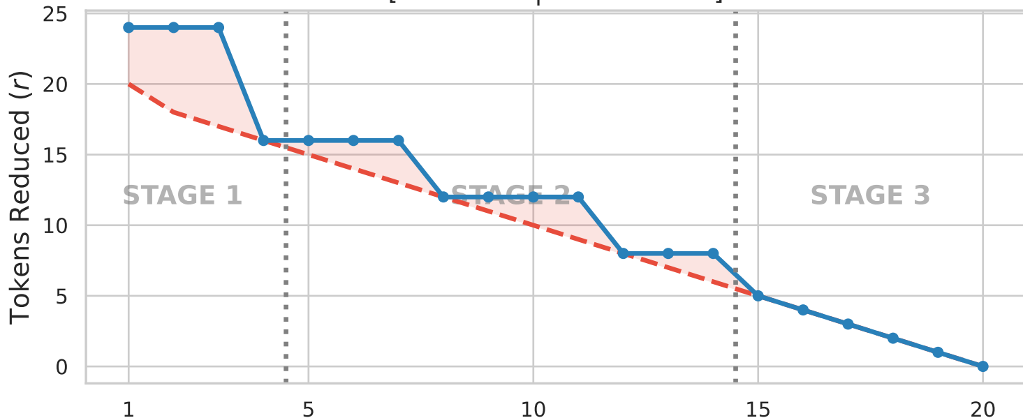
(b) Linear ( r_{lin} = 10 ) [Total: 223 | Acc: 74.64%]
