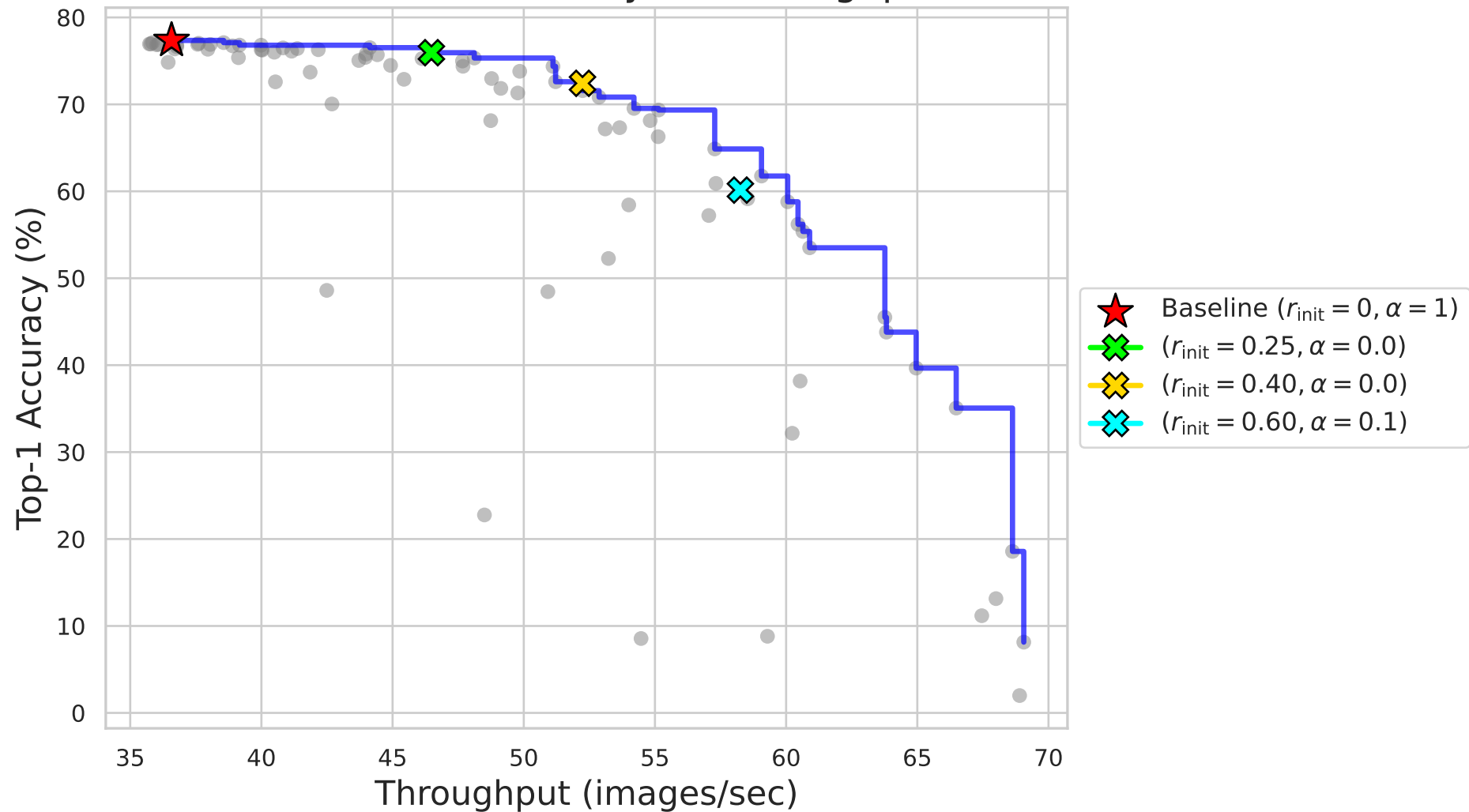
CPU Pareto Frontier: Accuracy vs. Throughput (BS=1)
