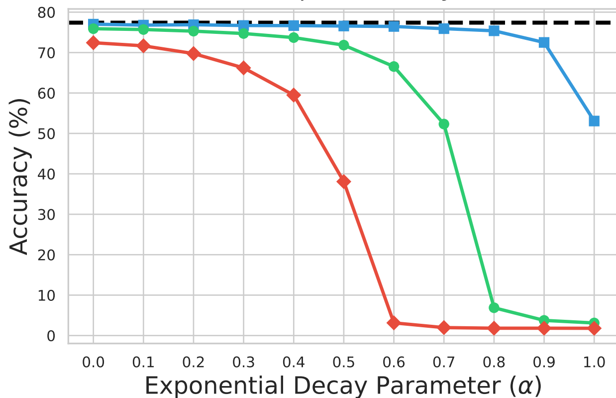
(a) Top-1 Accuracy
