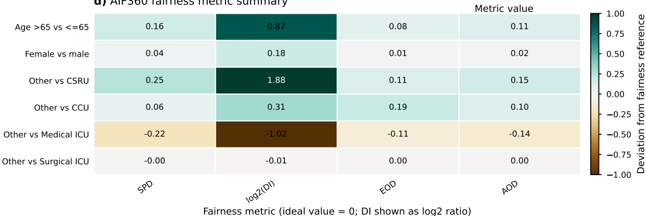
d) AIF360 fairness metric summary
