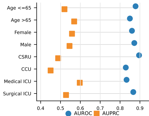
c) Subgroup predictive performance
