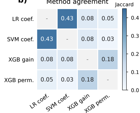
b) Method agreement
