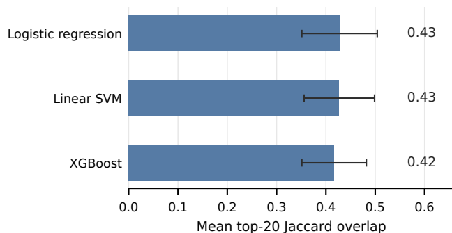
a) Cross-fold explanation stability
