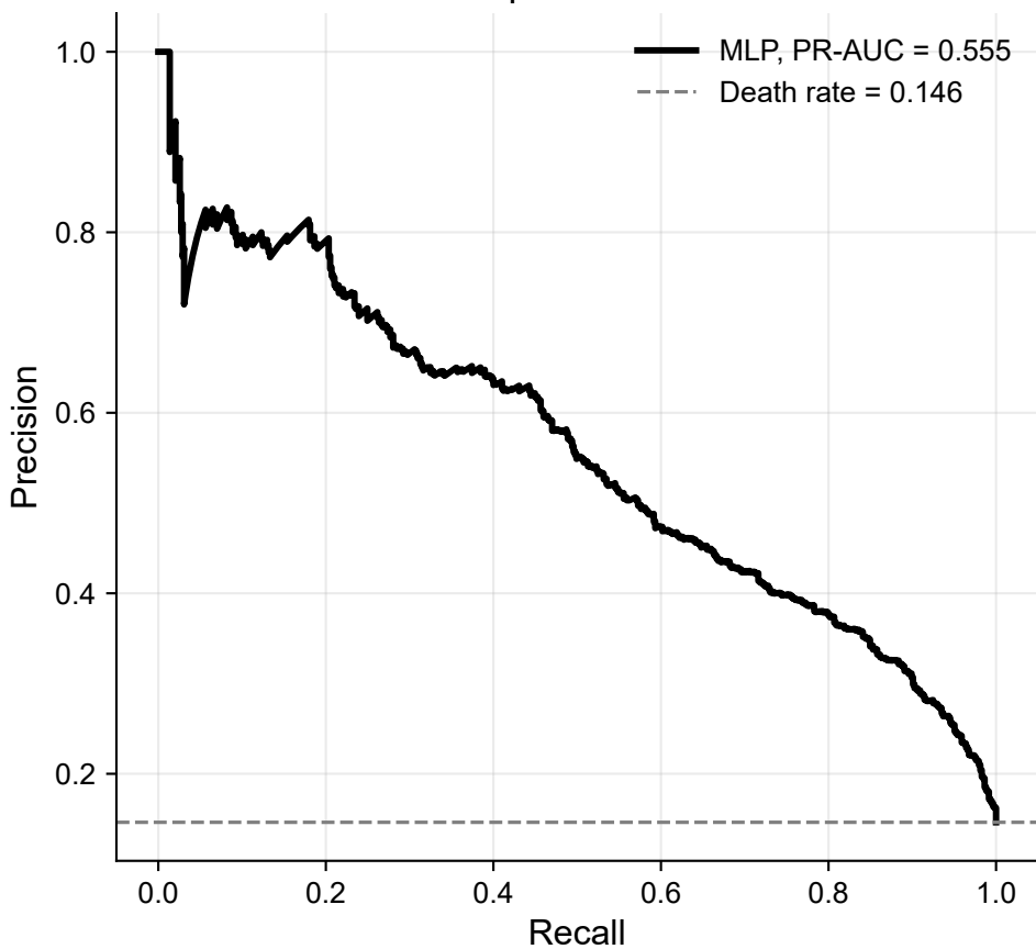
External test precision-recall curve
