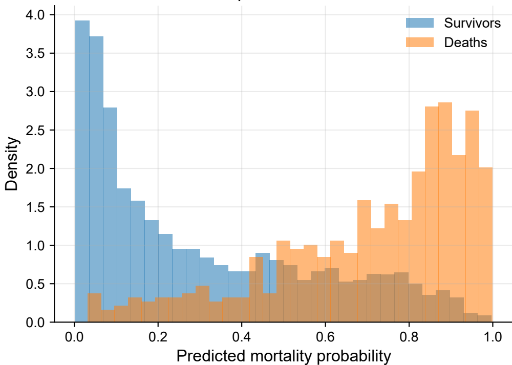
External test predicted risk distribution
