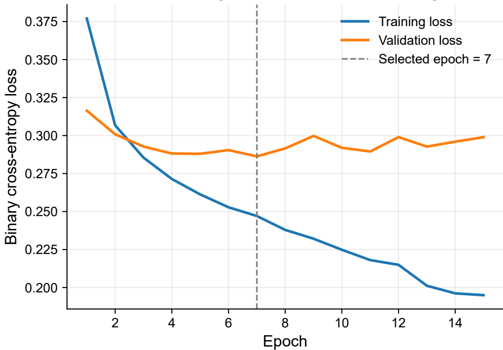
MLP training curve after validation tuning
