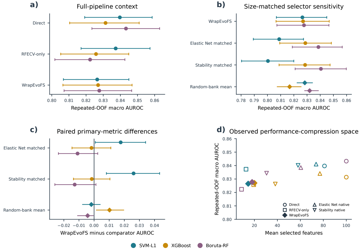
Figure 3. Fully nested TCGA performance and compression benchmark. All estimates use the same 491 participants, two stratified five-fold outer-CV repeats, training-only selection, and a fixed final random forest. Colors identify Direct branches. a) Repeated-OOF macro one-vs-rest AUROC for Direct, RFECV-only, and regret-constrained-medoid WrapEvoFS signatures. b) AUROC for WrapEvoFS, cardinality-matched Elastic Net and stability rankings, and five random-bank replicates summarized by their mean diamond and range. c) Paired AUROC differences between WrapEvoFS and each comparator; intervals for Elastic Net and stability selection use 2,000 participant-clustered class-stratified resamples, while random-bank symbols show the range across five prespecified replicate banks. d) Mean feature count versus AUROC for Direct, RFECV-only, WrapEvoFS, and native Elastic Net and stability supports. The selector-layer comparisons are conditional on the same post-Direct universe and do not establish standalone pipeline equivalence.
