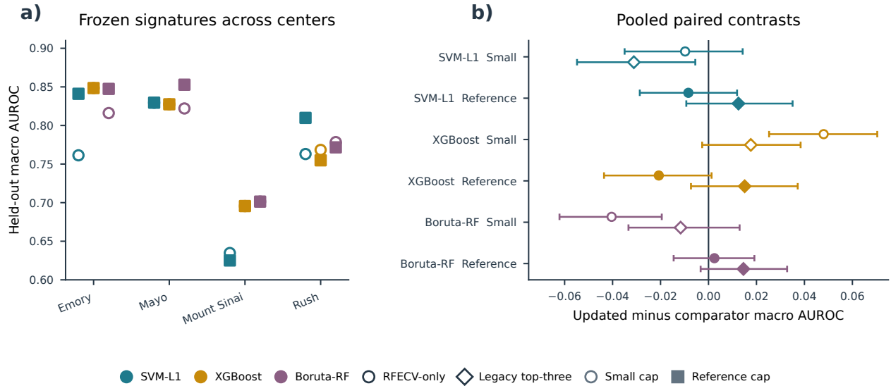
Figure 5. One-time post-freeze AMP-AD held-out evaluation. a) Macro one-vs-rest AUROC for 24 frozen signatures across combinations of center, branch, and cap; colors identify branches, open circles denote the Small cap, and filled squares denote the Reference cap. b) Pooled AUROC differences relative to RFECV-only (circles) and the legacy top-three medoid (diamonds), with 95% intervals from 2,000 common resamples stratified by held-out center and true class (seed 42). Open and filled symbols denote Small and Reference caps. All masks, parameters, and the protocol hash were frozen before held-out outcomes were loaded; evaluation triggered no reselection or retuning.
