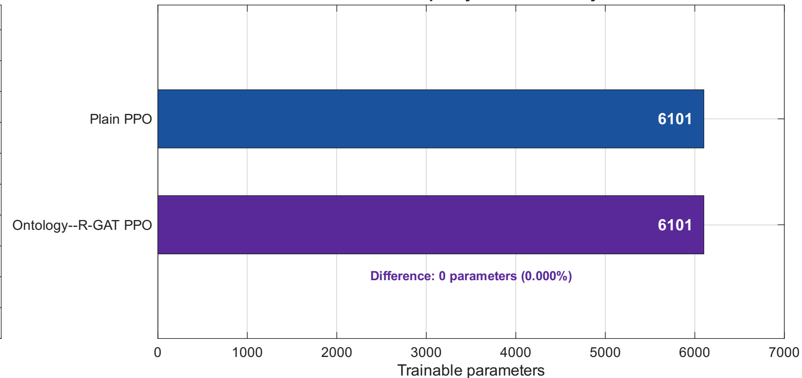
B Model capacity matched exactly
