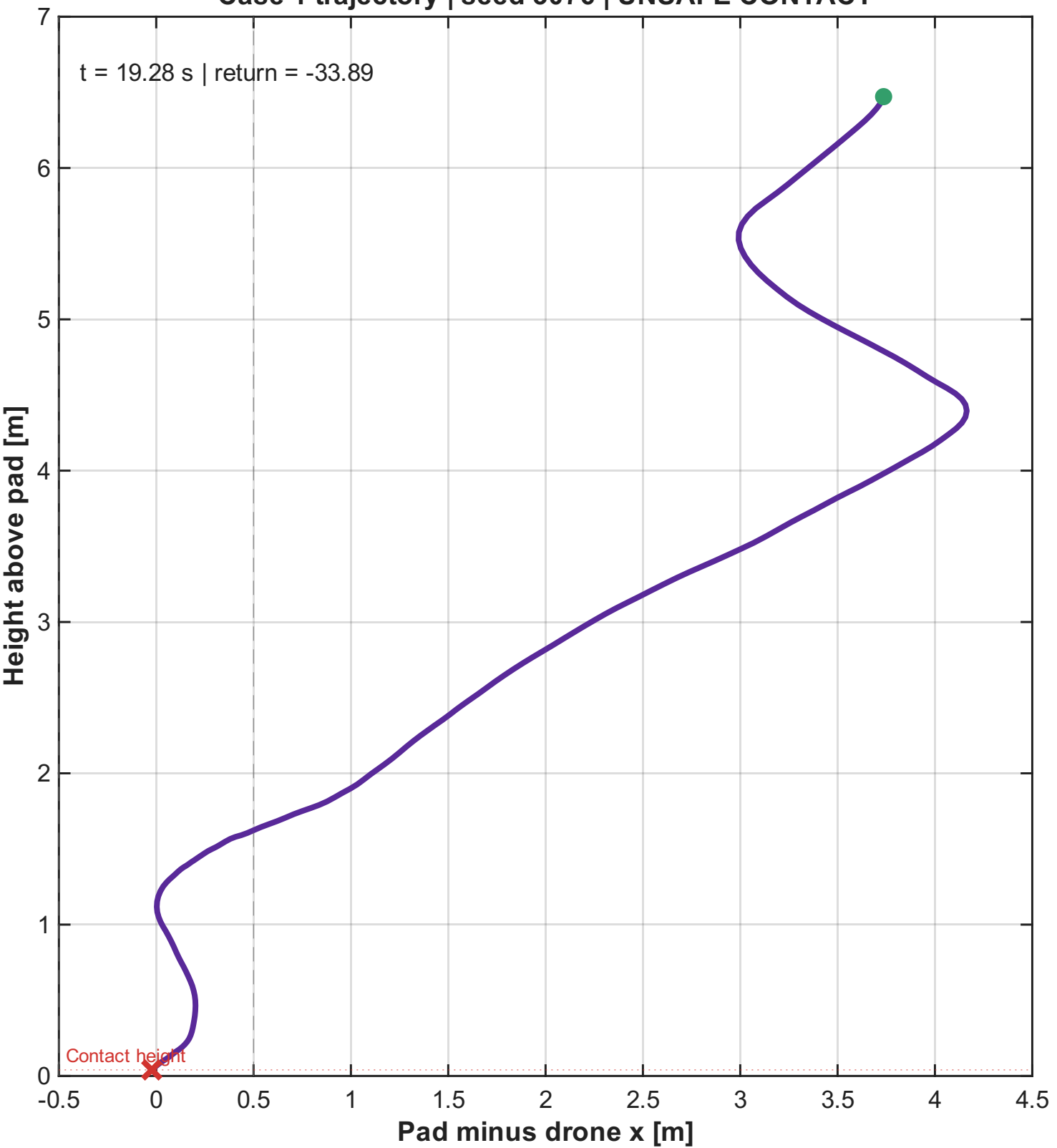
Case 1 trajectory | seed 3076 | UNSAFE CONTACT
