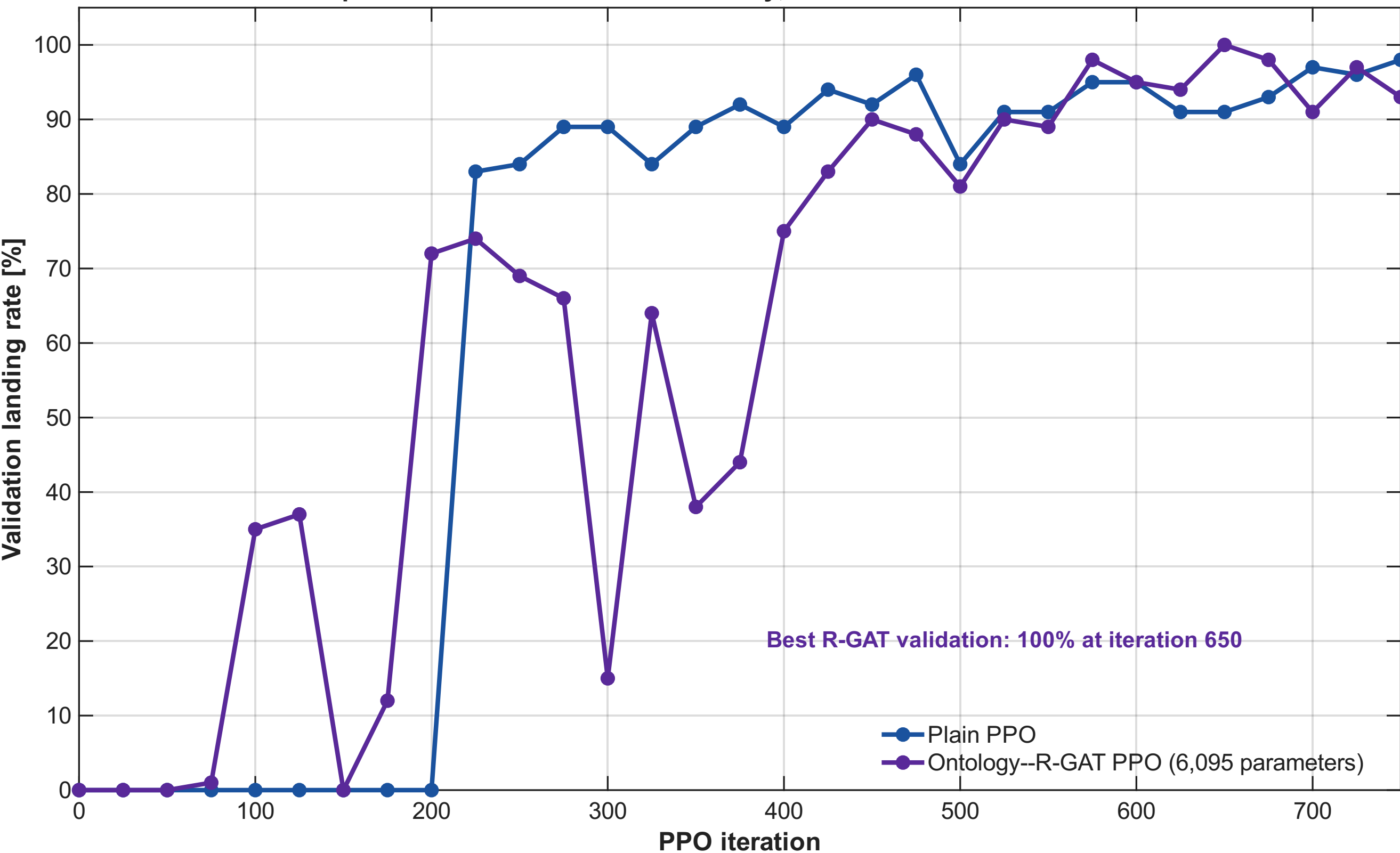
Validation learning curve under the same 4,500-episode budget Checkpoint selection uses validation only; held-out test seeds are never used
