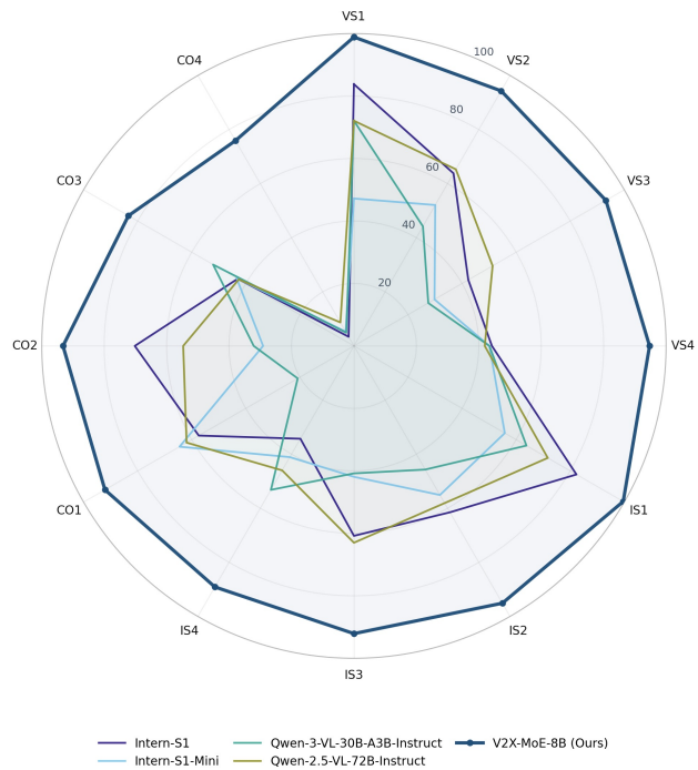
(b) Open-Source Model Performance Comparison
