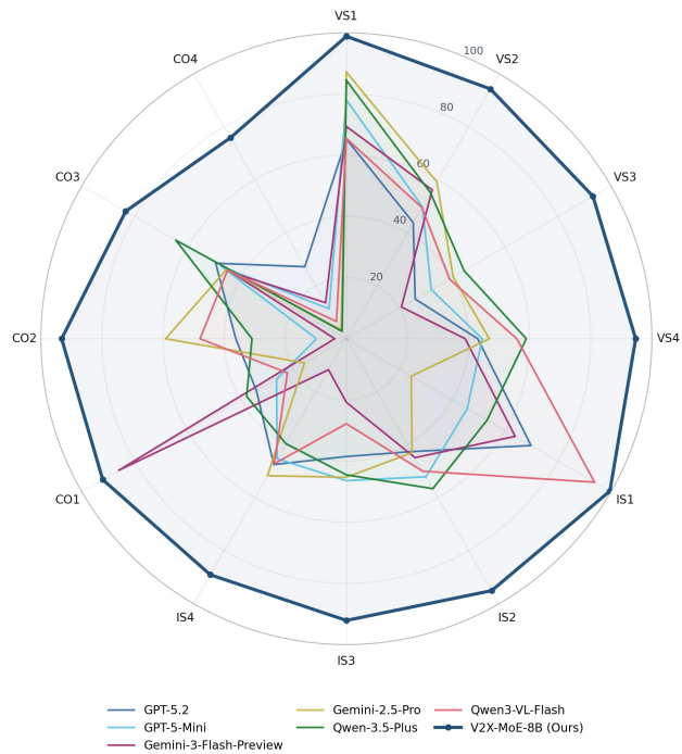
(a) Closed-Source Model Performance Comparison
